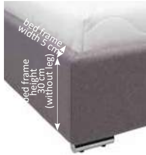
bed frame H (joined 45°)
