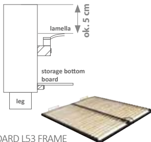
STANDARD L53 FRAME
