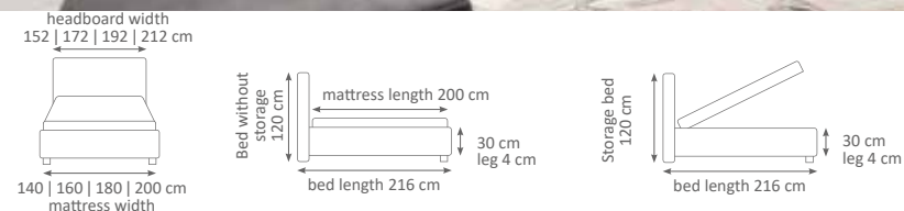
In the picture upholstered bed PORTO, leg B, fabric BELLAGIO AC 82, AQUACLEAN
