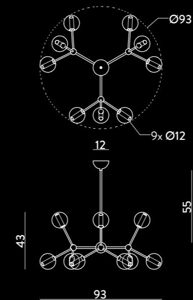
1574.9L LAMPADARIO / CHANDELIER Ø93 H 83 cm G9 9 x max 33W 230V IP20
