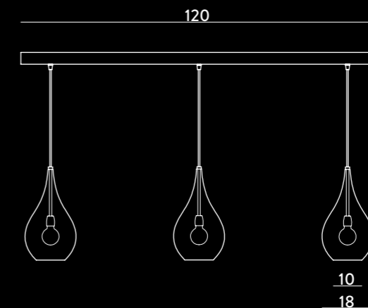
1257.120.3L BINARIO / CEILING TRACK Glass 3x Ø18 cm - cavo/cable 150 cm E14 3 x max 40W 220-240V CE IP20 1m
