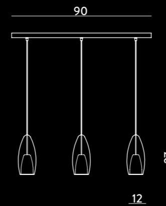
1397.90.3L BINARIO / CEILING TRACK Glass 3x Ø12 cm - cavo/cable 150 cm E14 3 x max 60W 220-240V C € IP20 1m
