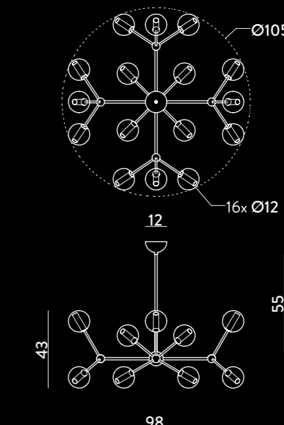
1574.12+4/16L LAMPADARIO / CHANDELIER Ø105 H 83 cm G9 16 x max 33W 230V IP20
