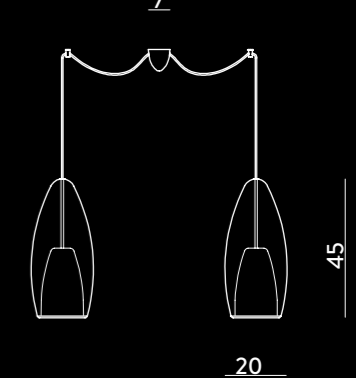
XXL1393.2L SOSPENSIONE / HANGING LAMP Glass 2x Ø20 cm - cavo/cable 250 cm E27 2 x max 105W 220-240V C € IP20 1m
