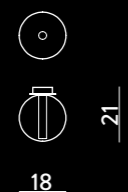
1576.18.1L PLAFONIERA / CEILING LAMP Ø18 x H 21 cm G9 1 x max 33W 230V IP20
