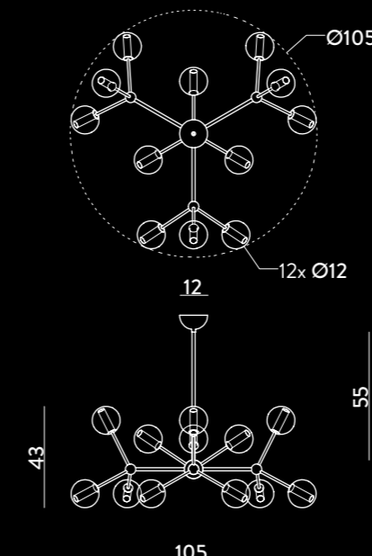
1574.9+3/12L LAMPADARIO / CHANDELIER Ø105 H 83 cm G9 12 x max 33W 230V IP20
