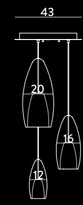
1399MX.43.3L PLAFONIERA / CEILING LAMP Glass Ø12/16/20 cm - cavo/cable 150 cm E14 1 x max 60W 220-240V E27 2 x max 105W 220-240V C € IP20 1m
