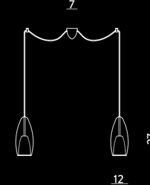
1393.2L SOSPENSIONE / HANGING LAMP Glass 2x Ø12 cm - cavo/cable 250 cm E14 2 x max 60W 220-240V C € IP20 1m
