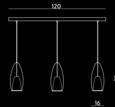
GIG1397.120.3L BINARIO / CEILING TRACK Glass 3x Ø16 cm - cavo/cable 150 cm E27 3 x max 105W 220-240V C € IP20 1m
