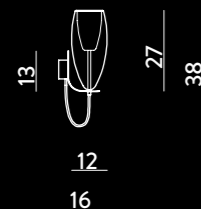
AP1391.1L APPLIQUE / WALL LAMP Glass Ø12 cm - cavo/cable 50 cm E14 1 x max 60W 220-240V C € IP20 1m
