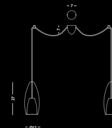
1393.2L Sospensione / Hanging lamp vetro/glass Ø12 cm - cavo/cable 250 cm 💡 2 E14 x max 60W 220-240V C E IP20 (1m)
