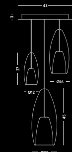
1399MX.43.3L Plafoniera / Ceiling lamp vetro/glass Ø12/16/20 cm - cavo/cable 150 cm 💡 2 E27 x max 105W 💡 1 E14 x max 60W 220-240V C E IP20 (1m)
