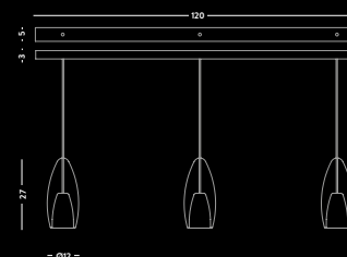
1397.120.3L Binario a soffitto / Ceiling track vetro/glass Ø12 cm - cavo/cable 150 cm 💡 3 E14 x max 60W 220-240V C E IP20 (1m)
