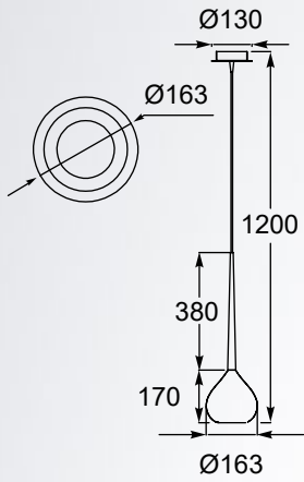
LIBRA Pendant lamp MD2128-1W 1xE14 MAX 40W metal chrome canopy, black metal body, white glass shiny shade
