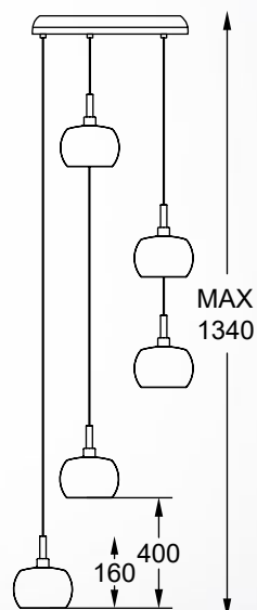
CRYSTAL Pendant lamp P0076-05M-B5FZ 5xG9 MAX 42W smoky chrome glass shade clear crystal drops inside
