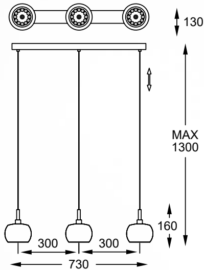
CRYSTAL Pendant lamp P0076-03N-B5FZ 3xG9 MAX 42W smoky chrome glass shade clear crystal drops inside
