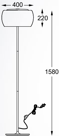
CRYSTAL Floor lamp P0076-04A-F4FZ 4xG9 MAX 42W smoky chrome glass shade clear crystal drops inside
