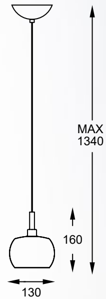
CRYSTAL Pendant lamp P0076-01A-F4FZ 1xG9 MAX 42W smoky chrome glass shade clear crystal drops inside
