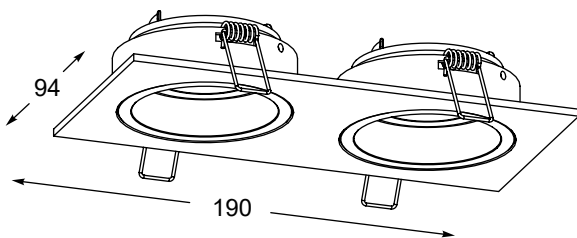
CHUCK DL2 SQUARE Spot 1. 20068-BK (black) 2. 20068-WH (white) 2xGU10 MAX 50W aluminium white or black
