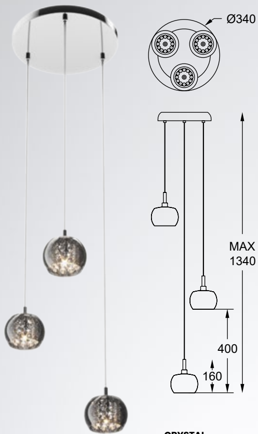
CRYSTAL Pendant lamp P0076-03M-B5FZ 3xG9 MAX 42W smoky chrome glass shade clear crystal drops inside
