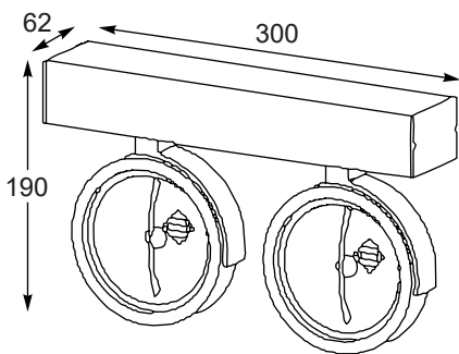
GO SL 2 Spot 1. 89964 (white) 2. 50485 (black) 2xG9 MAX 42W aluminium white or black
