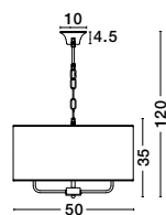
Elizabeth 8120041 Antique Bronze Metal Sand Shade E14 4x40 Watt 230 Volt IP20 Bulb Excluded D: 50 H1: 35 H2: 120 cm
