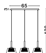
Boccale 1300301303 Chrome Aluminium Clear Glass G9 3x33 Watt 230 Volt IP20 Bulb Included L: 65 W: 10 H: 120 cm
