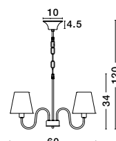
Elizabeth 7120022 Antique Bronze Metal Sand Shade E14 5x40 Watt 230 Volt IP20 Bulb Excluded D: 60 H1: 34 H2: 120 cm
